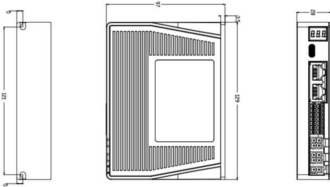
2DM3-EC432S: 长*高*宽: 129*97*28 (mm)
