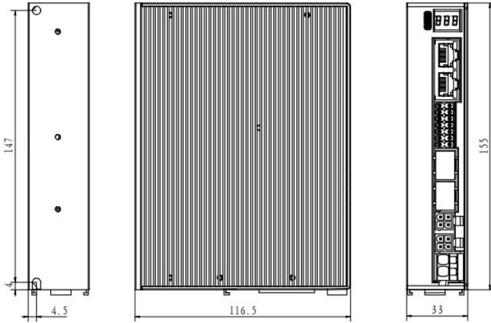
2DM3-EC882S: 长*高*宽: 155*116.5*33 (mm)
